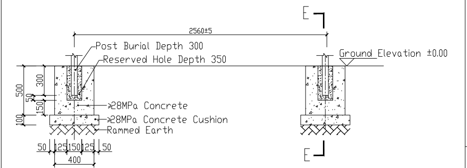
Foundation Elevation
