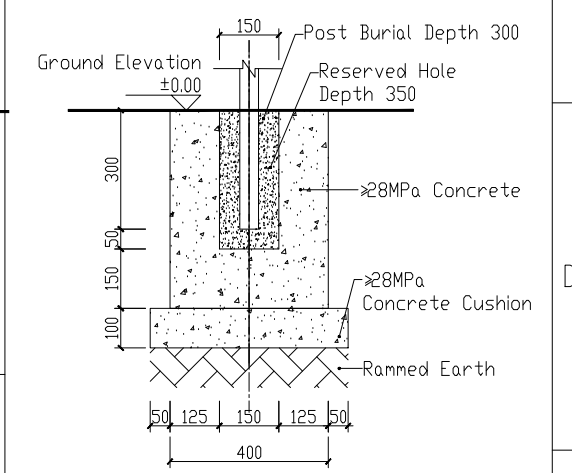
E-E Sectional 2:1
