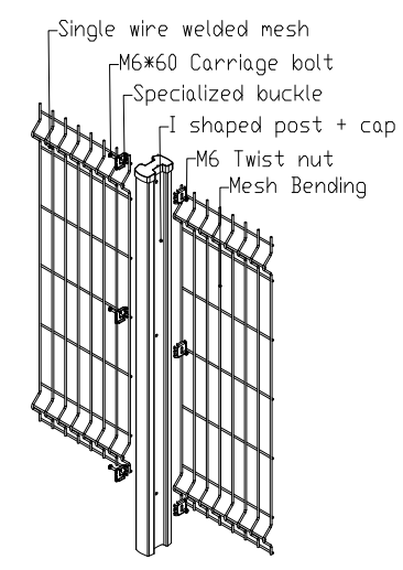
Fence Perspective
